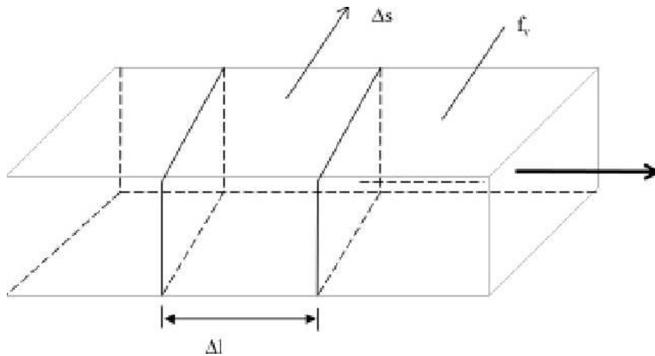
Fig: Current in a filament
